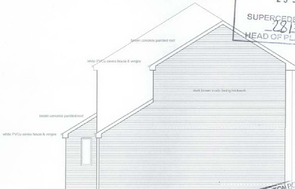
Gable End Elevation (proposed)
